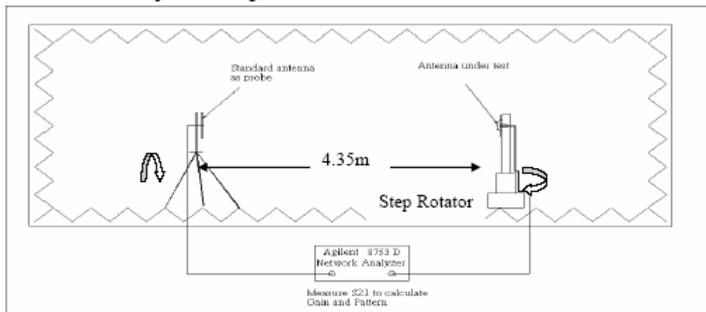
Fig.2 The interior components of the anechoic chamber
