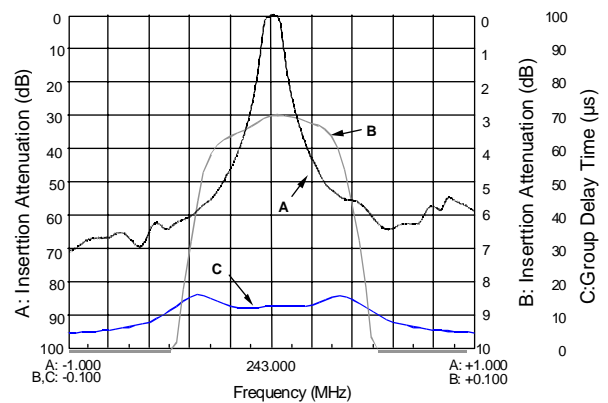
HF-363A 243 MHz
